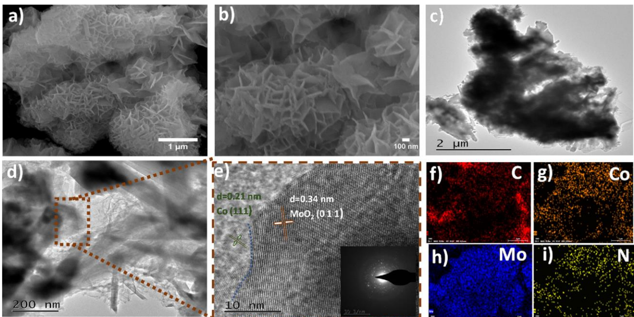
Fig. 2 The morphology and crystal structure of CMO@NC/450 sample: (a, b) SEM, TEM and HR-TEM images (inset showed corresponding SAED pattern); images; (d-e) and (f-i) EDS elemental mapping (Scale bar: 2 μm). Reproduced with permission from Ref.[18] (Copyright 2020, Elsevier B.V.).
