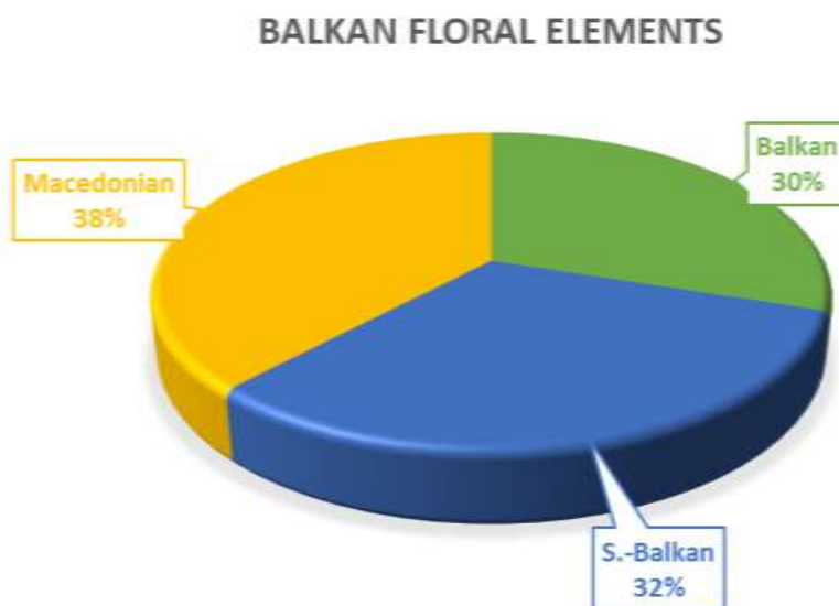
Figure 7. ass. Cynosureto-Caricetum hirtae galietosum macedoniceae subass. nova – Balkan floral elements
